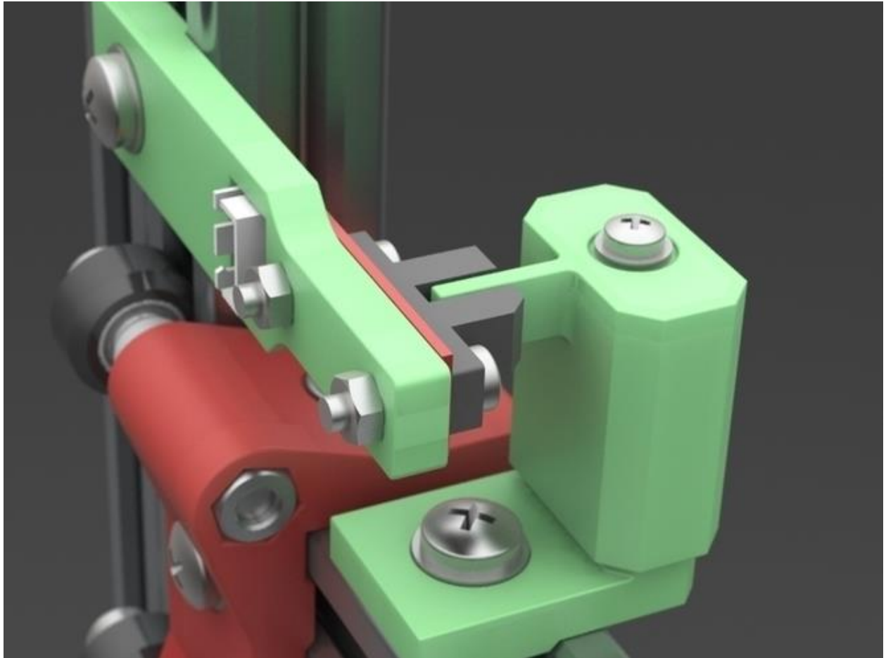
End Stop Detection in 3-D Printer.
